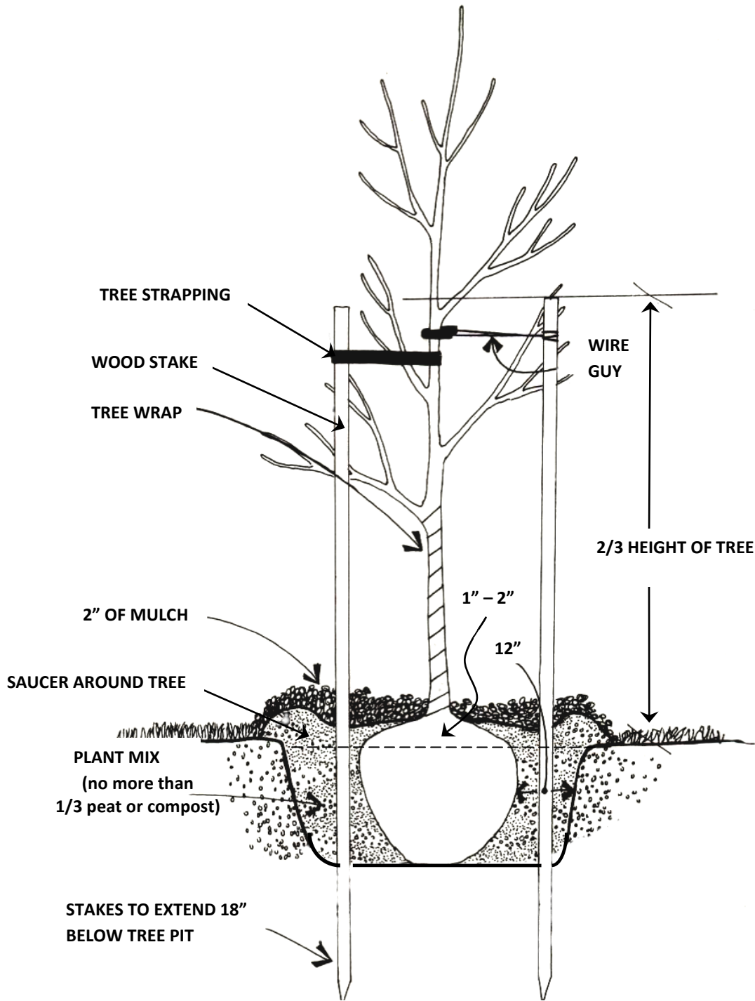
TYPICAL TREE PLANTING DETAIL FOR TREES WITH A CALIPER LESS THAN 3"
